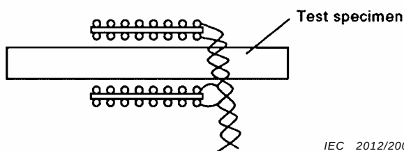
Figure 5d – Field-sensing coils (H-coils), flat type – two coils connected in series addition
