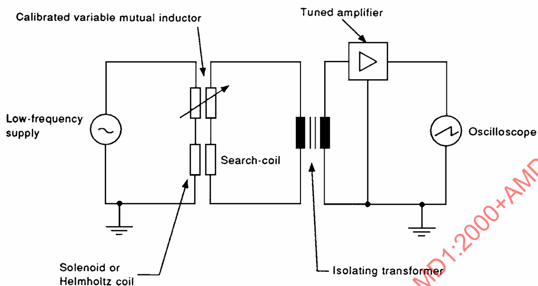
Figure A.1 – Circuit for the calibration of search-coils
