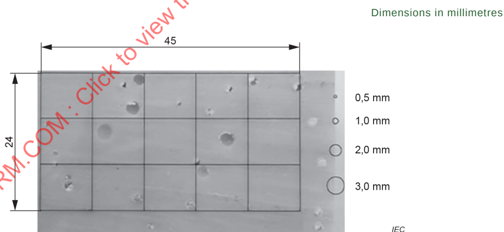
Figure A.2 – Position of examination grid on the specimen
