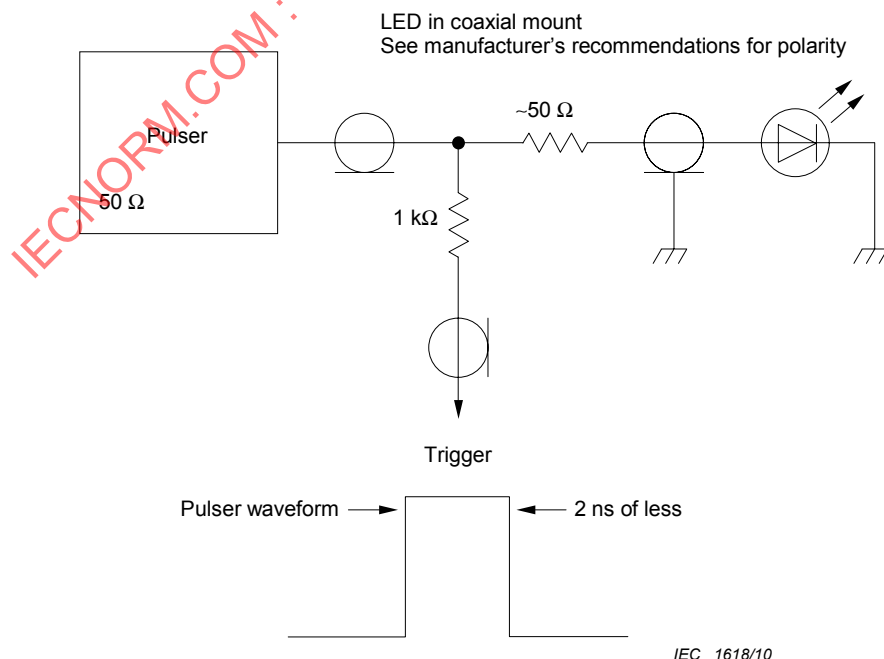
Figure A.1 – Light-emitting diode circuitry
