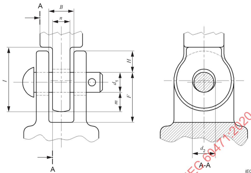
Figure 2 – Dimensions of clevis and tongue couplings for long rod insulators
