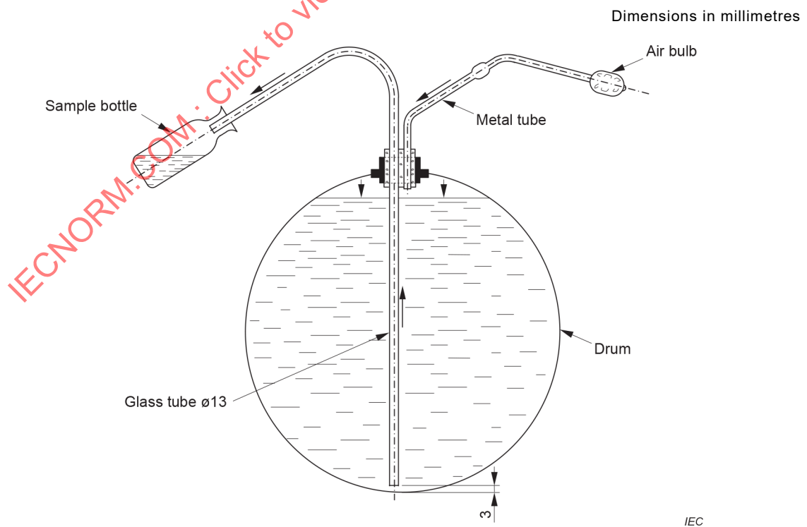
Figure 4 – Siphon
