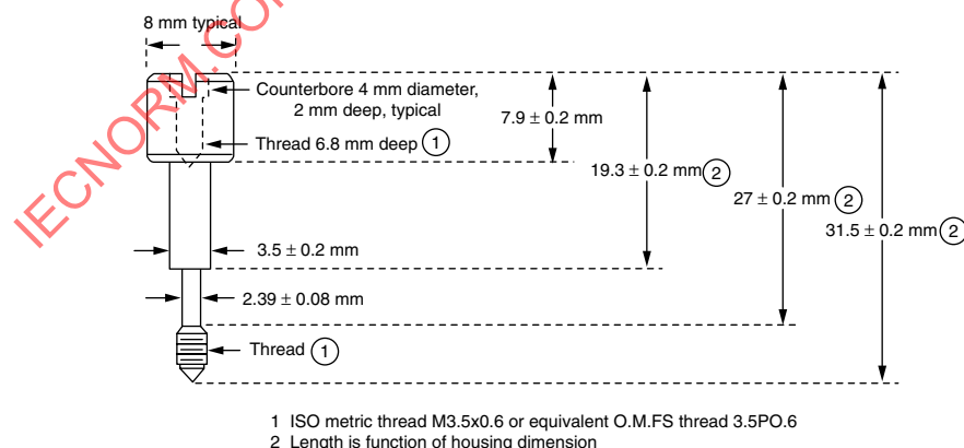
Figure 23—Lock screw
