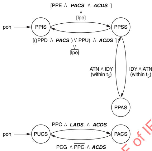
Figure 13—PP state diagram
