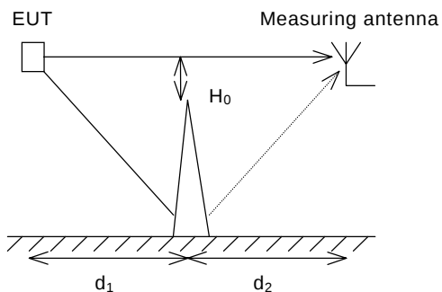
Figure A.6a – Radio-wave screening curtain
