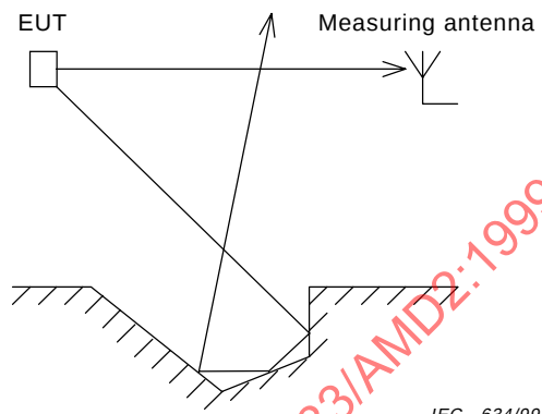
Figure A.6b – Mazed gap
