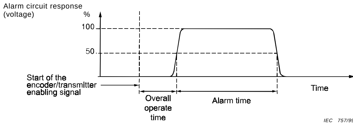
Figure 19 – System overall operate and alarm time
