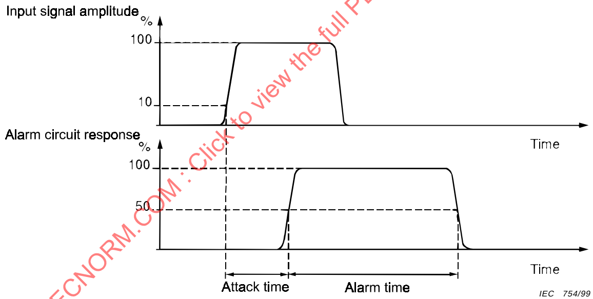
Figure 16 – Decoder attack time
