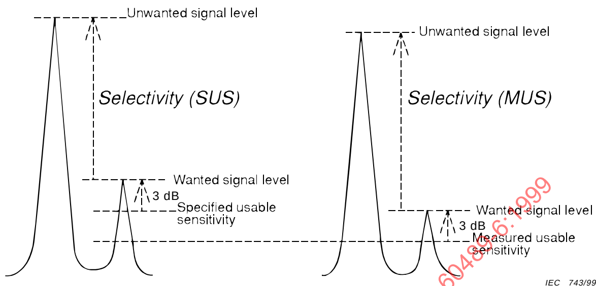
Figure 5a – Selectivity measurement using specified usable sensitivity
