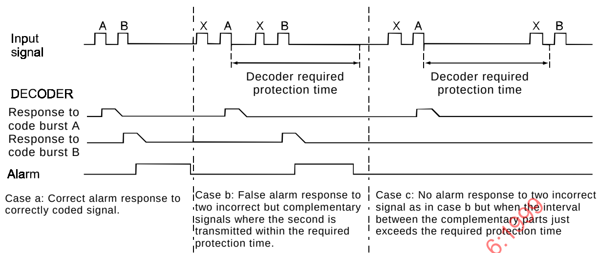
Figure 17 – Decoder required protection time
