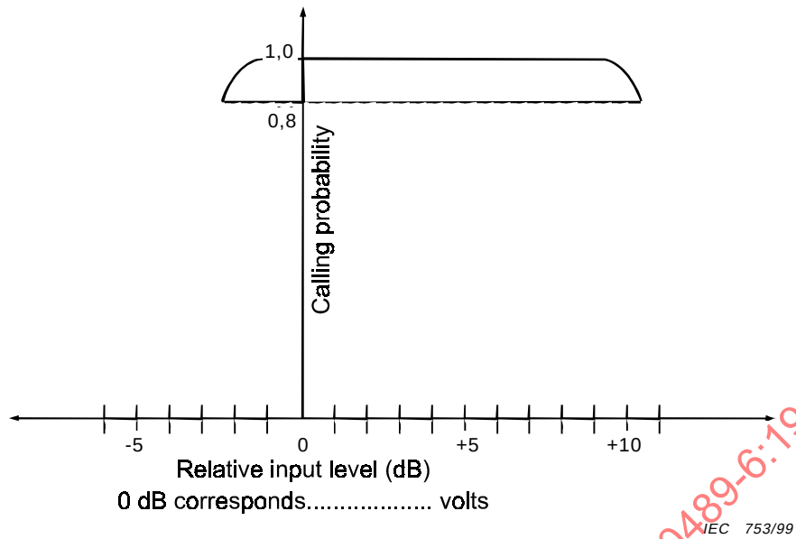
Figure 15 – Decoder operation level range
