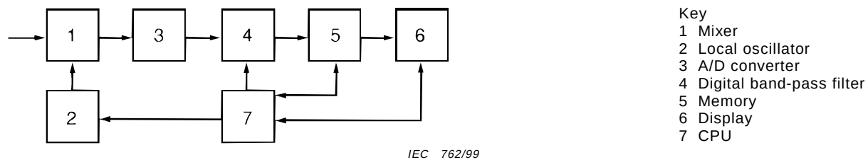
Figure B.1 – Example of power measuring receiver with a digital band-pass filter
