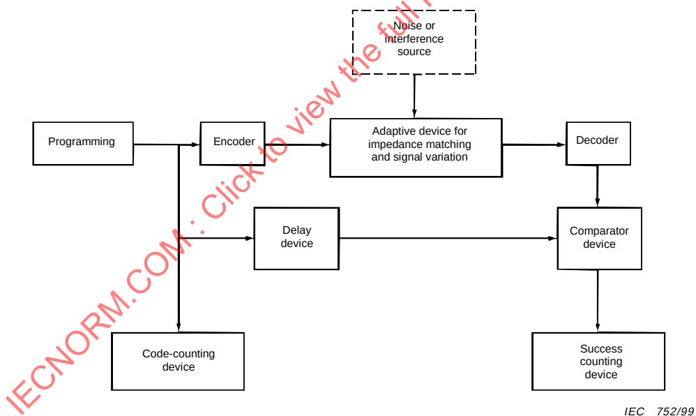
Figure 14 - Typical measurement arrangement
