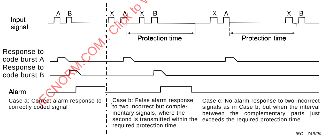
Figure 8 – Protection time
