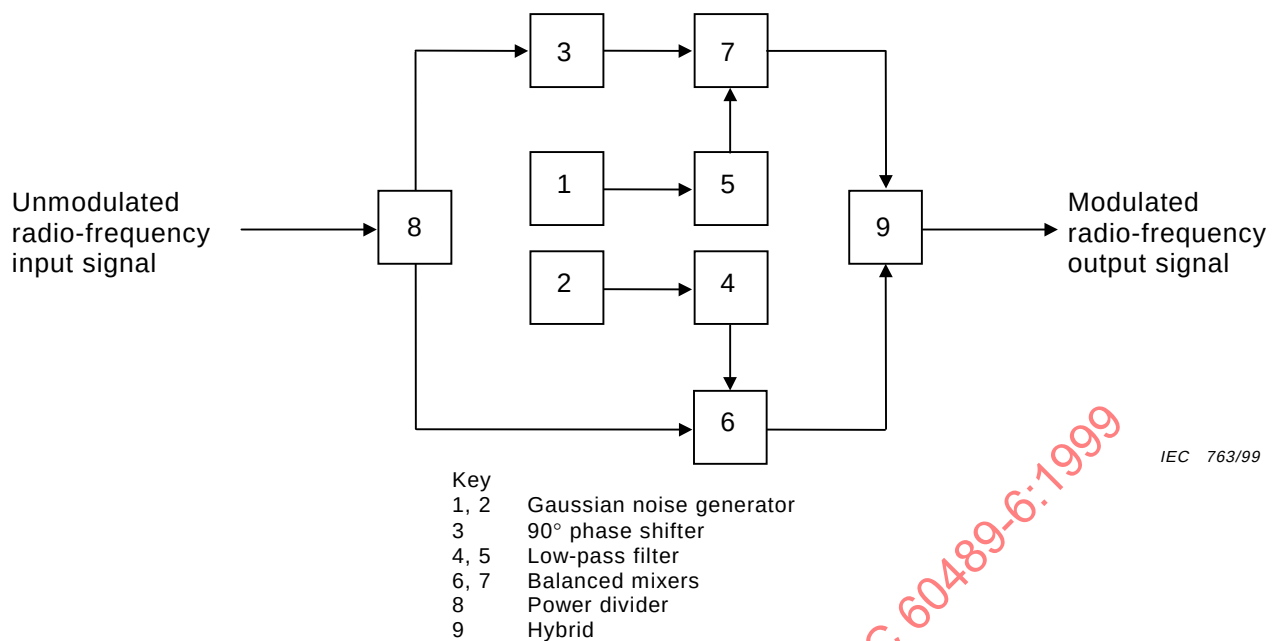
Figure C.1 – Example of a Rayleigh fading simulator
