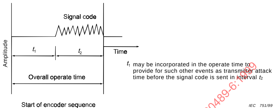
Figure 13 – Encoder overall operate time
