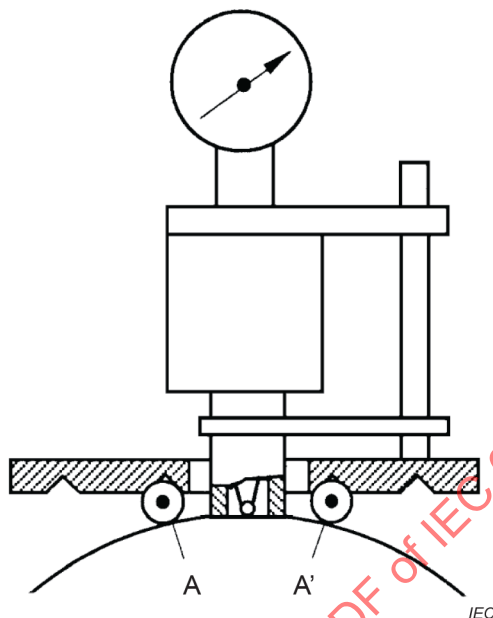
Figure C.1 – Test on surfaces of large radius of curvature
