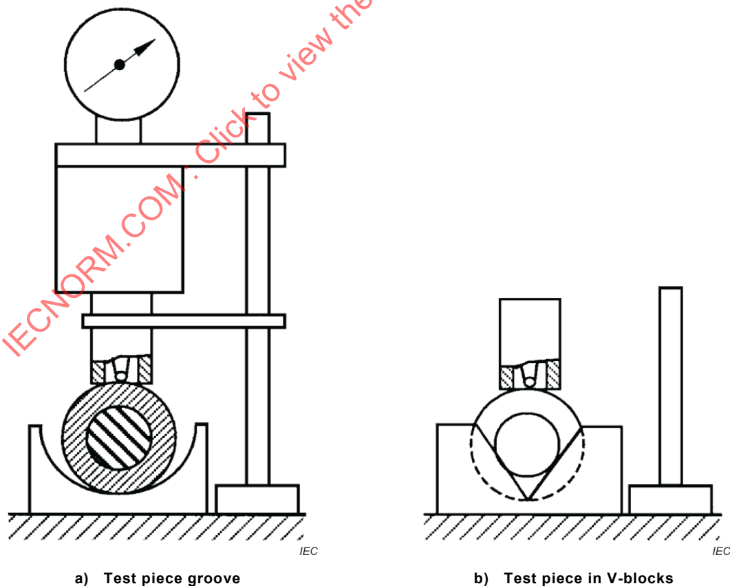
Figure C.2 – Test on surfaces of small radius of curvature
