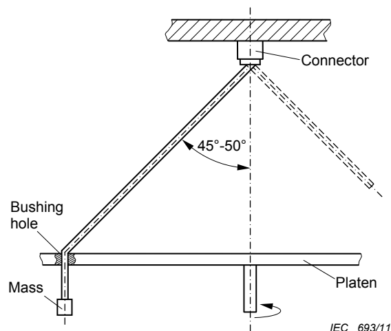
Figure 1 – Cable test set-up
