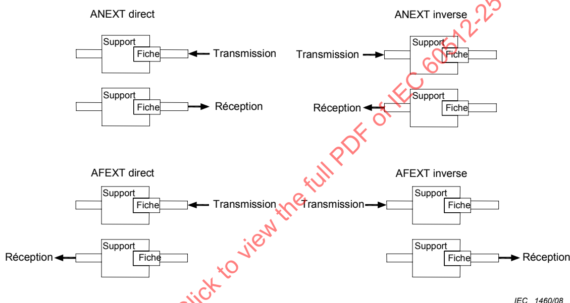
Figure 4 – Directions d'essai
