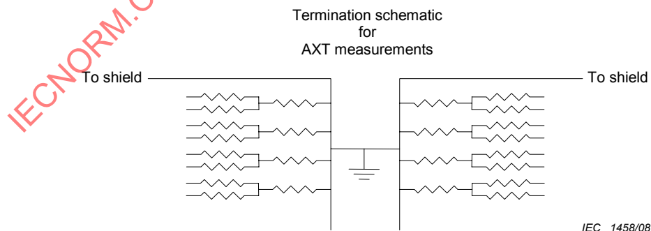
Figure 2 – Schematic for terminations
