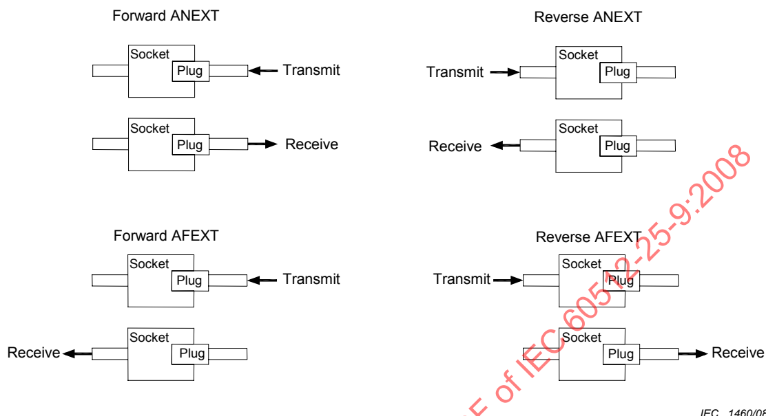
Figure 4 – Test directions
