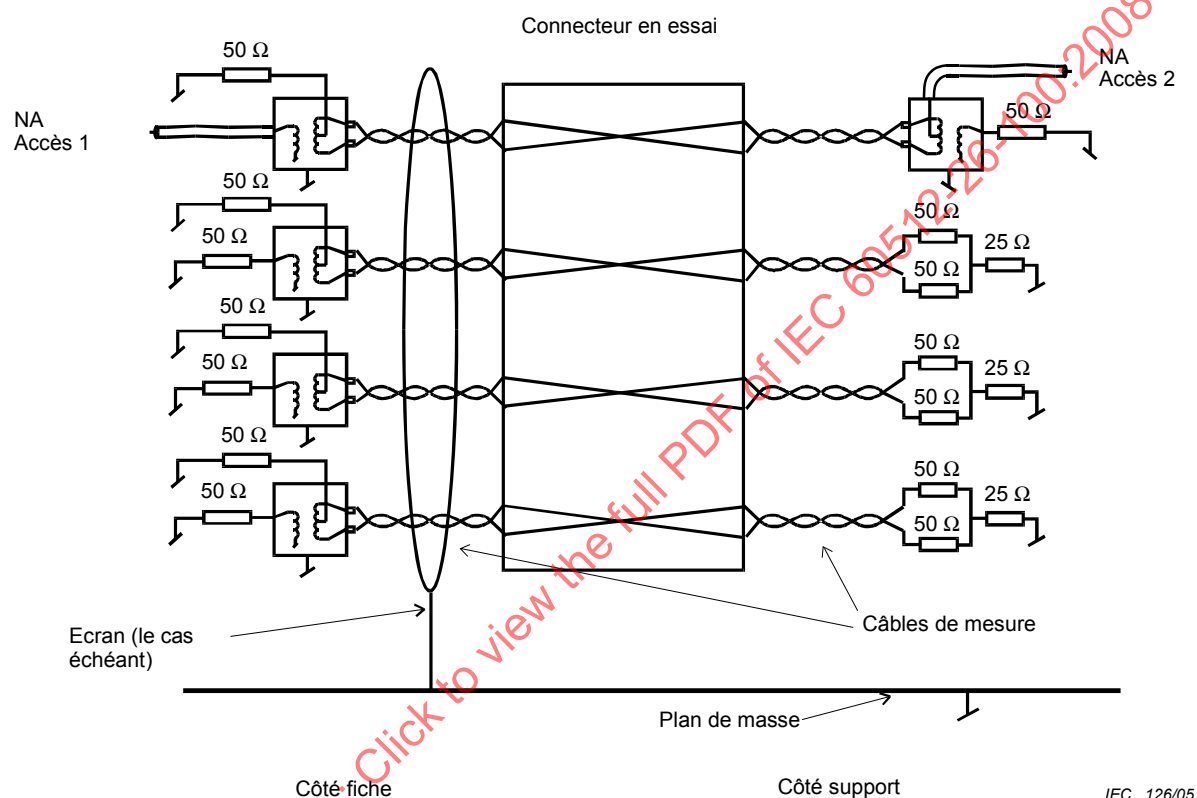
Figure 16 – Mesure TCTL
