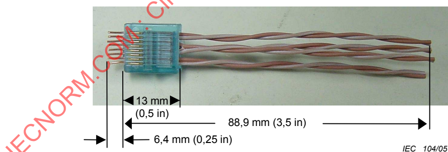
Figure 21 – De-embedding reference FEXT plug without sockets
