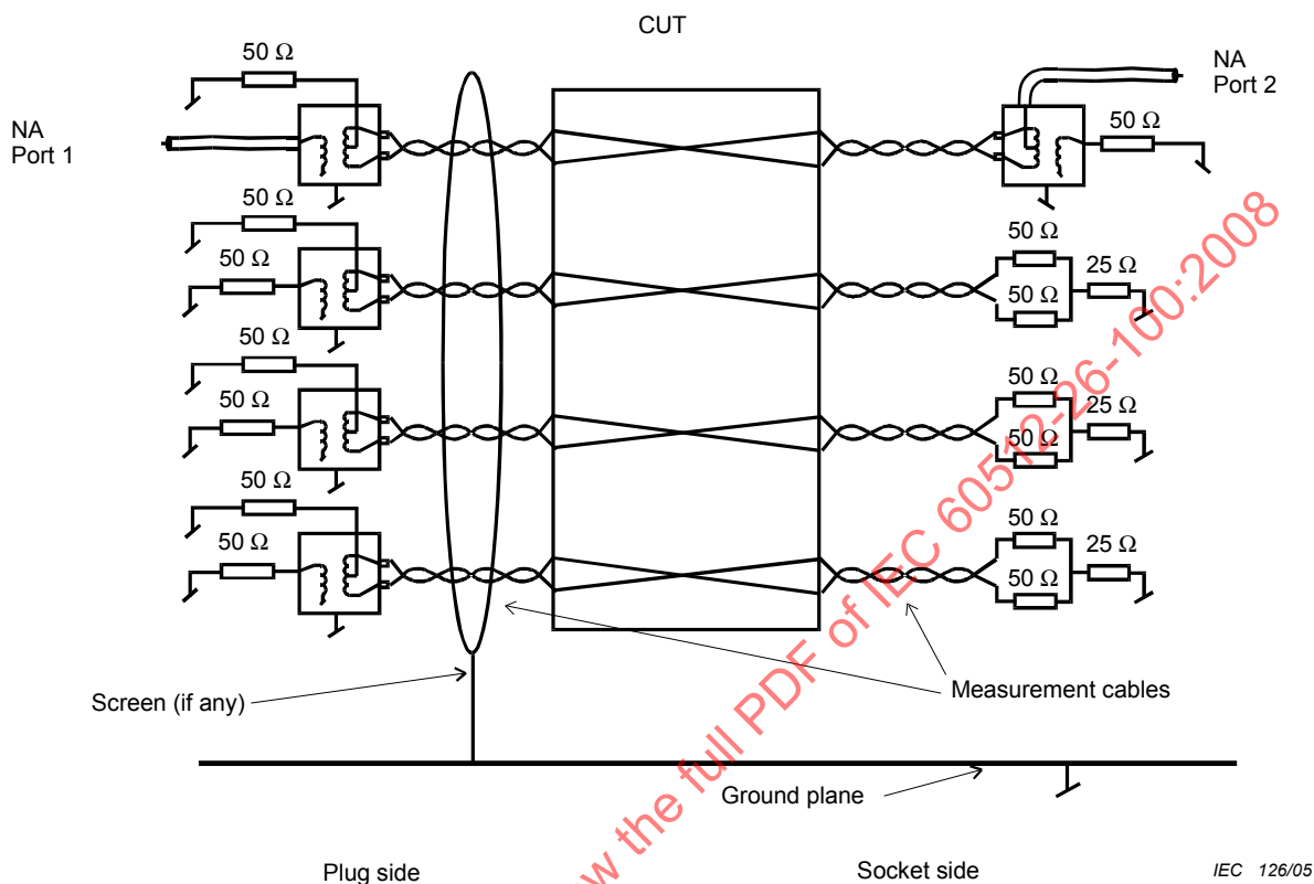
Figure 16 – TCTL measurement
