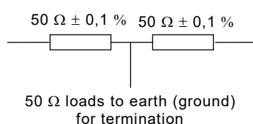
Figure 4 – Resistor termination networks
