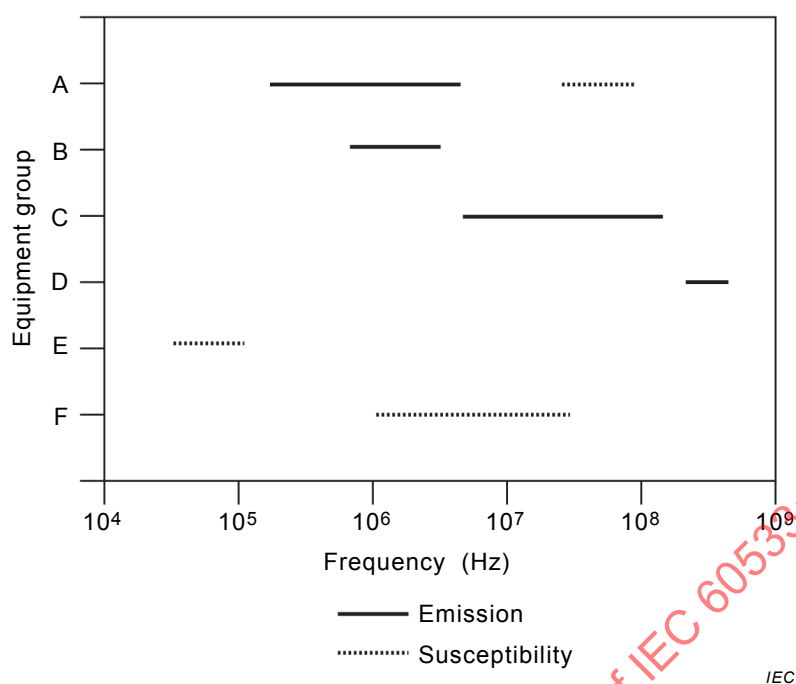
Figure A.3 – EMC analysis, frequency survey
