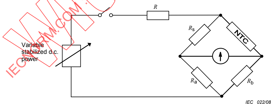
Figure 4 – Zero-power resistance measuring basic circuit
