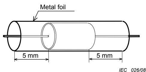
Figure 8 – Test method 3
