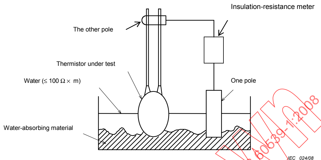
Figure 6 – Test method 2
