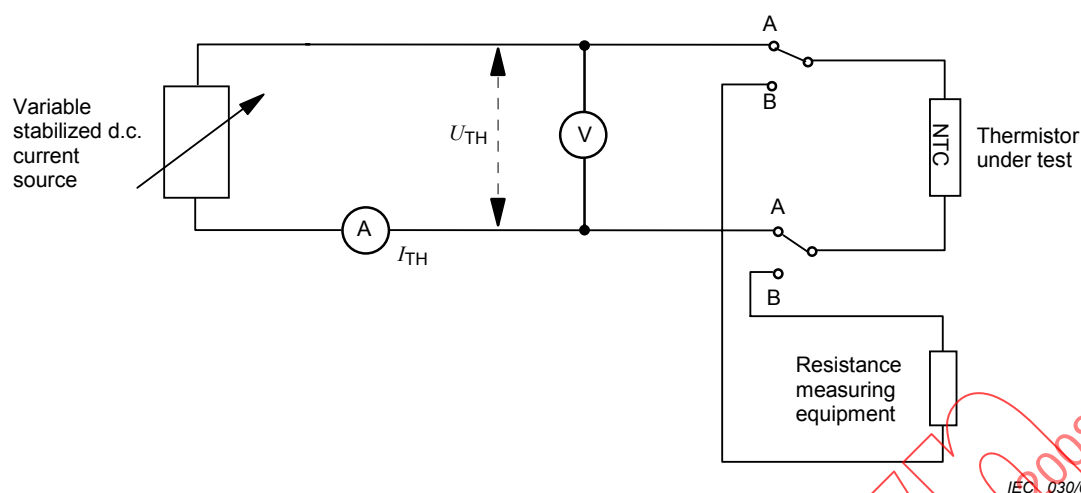
Figure 12 – Thermal time constant measuring circuit
