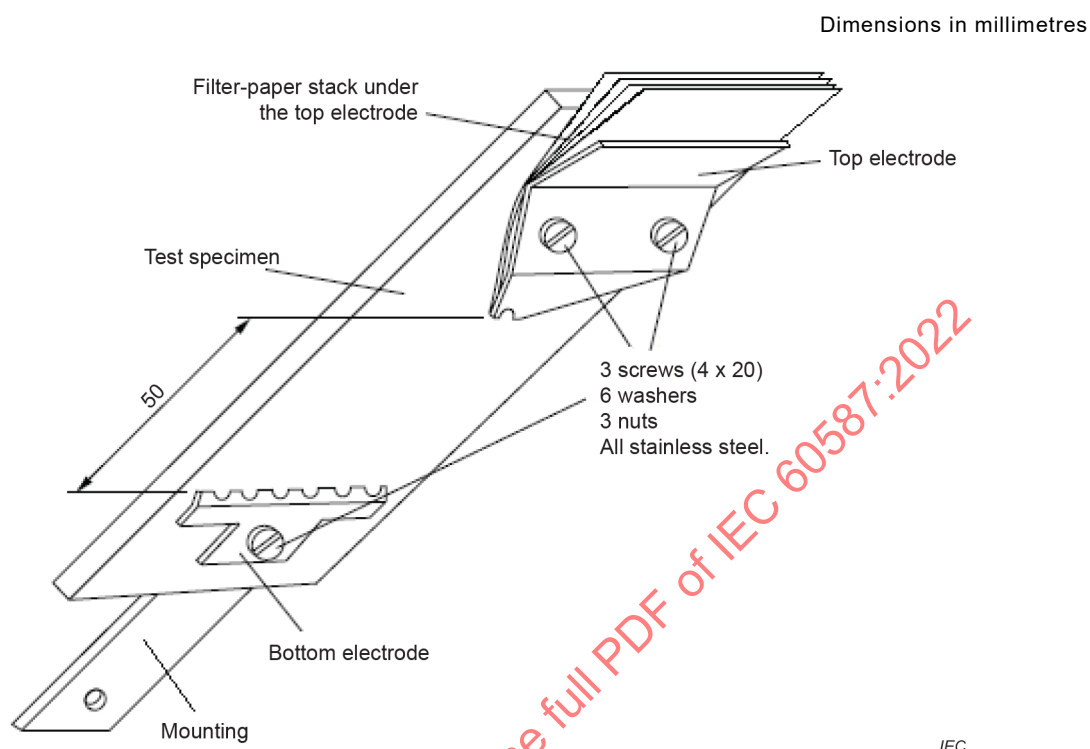
Figure 4 – Schematic diagram of specimen assembly
