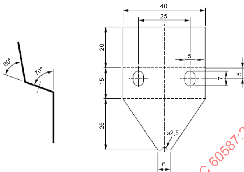
Figure 5 – Electrode supérieure
