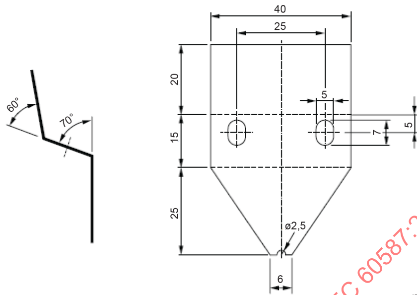
Figure 5 – Top electrode
