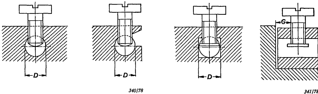
Bornes sans plaquette Terminals without pressure plate
