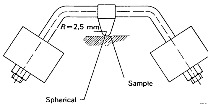
Figure 10 – Ball-pressure apparatus
