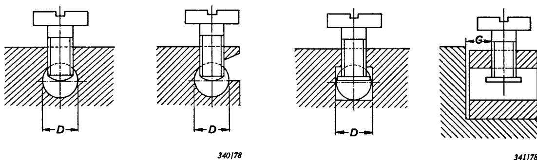
Bornes sans plaque
