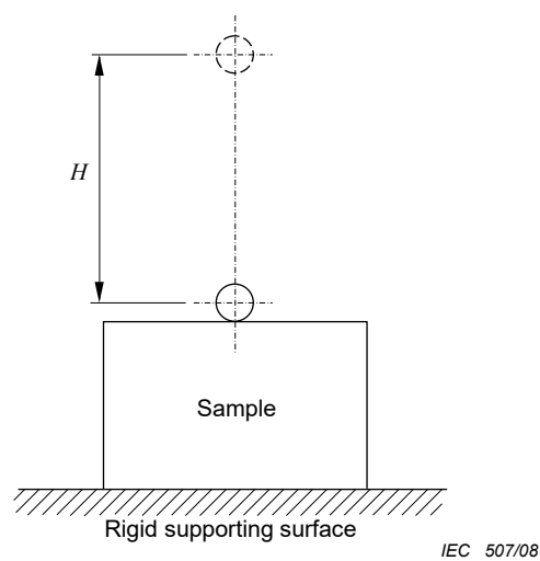
Figure 21 – Apparatus for ball impact tests
