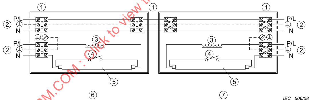
c) Illustration of the term "through wiring" not terminating in the luminaire
