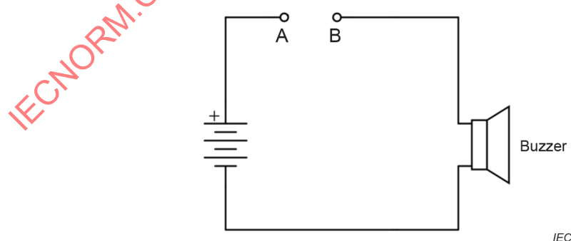
Figure 34 – Circuit for checking electrical contact between socket outlet and plug
