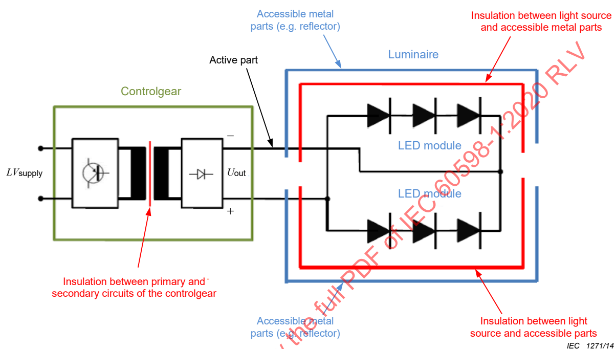
Figure X.1 – Declaration of LV_{supply} and U_{out} and the insulation barriers between the light source and accessible parts
