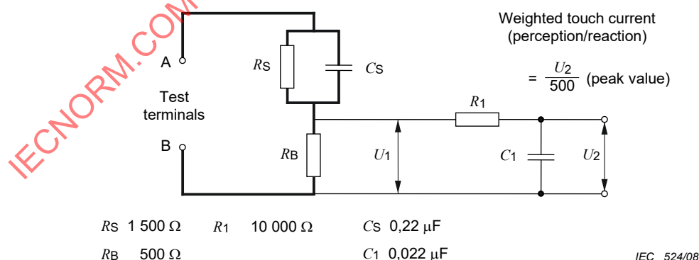
Figure G.2 – Measuring network, touch current weighted for perception or reaction
