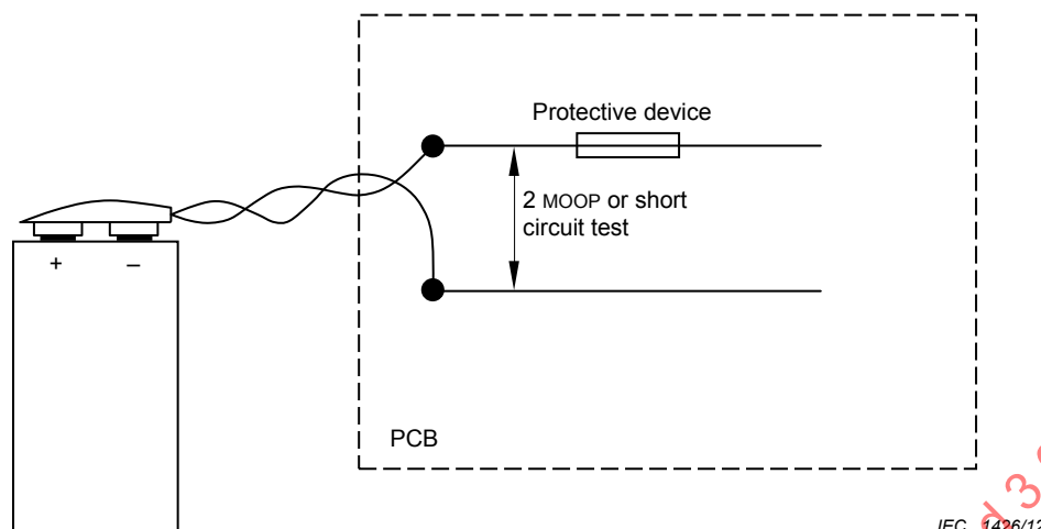
Figure A.23 – Example of the needed MEANS OF OPERATOR PROTECTION between the terminals of an INTERNAL ELECTRICAL POWER SOURCE and a subsequent protective device
