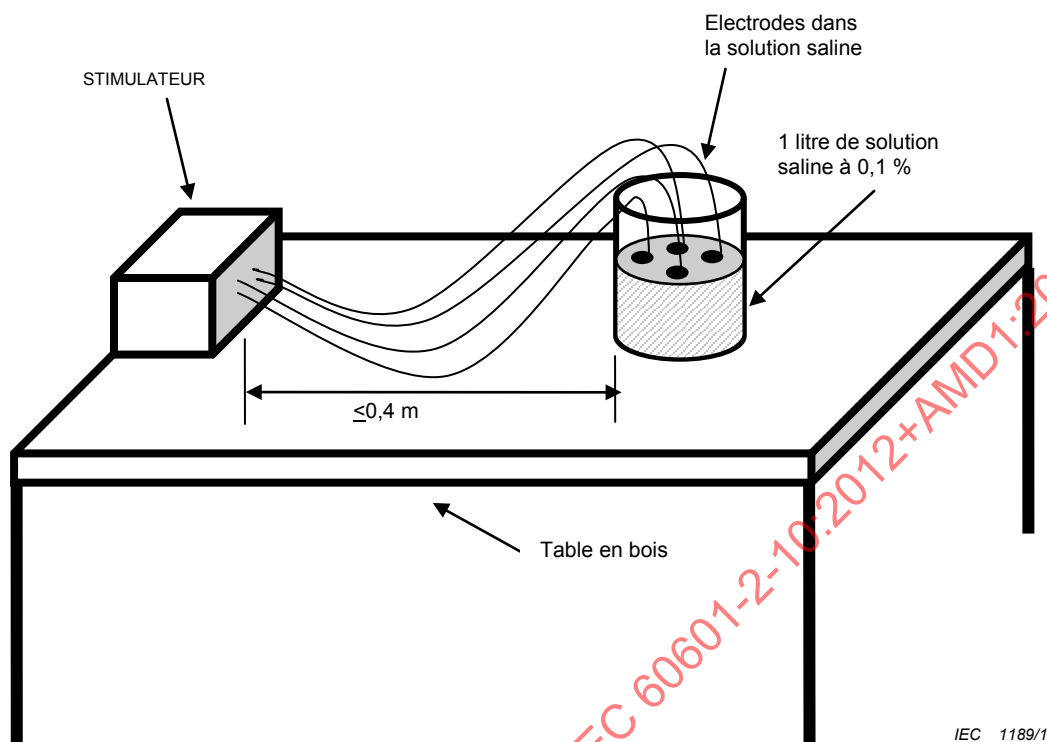
Figure 202.101 – Installation d'essai
