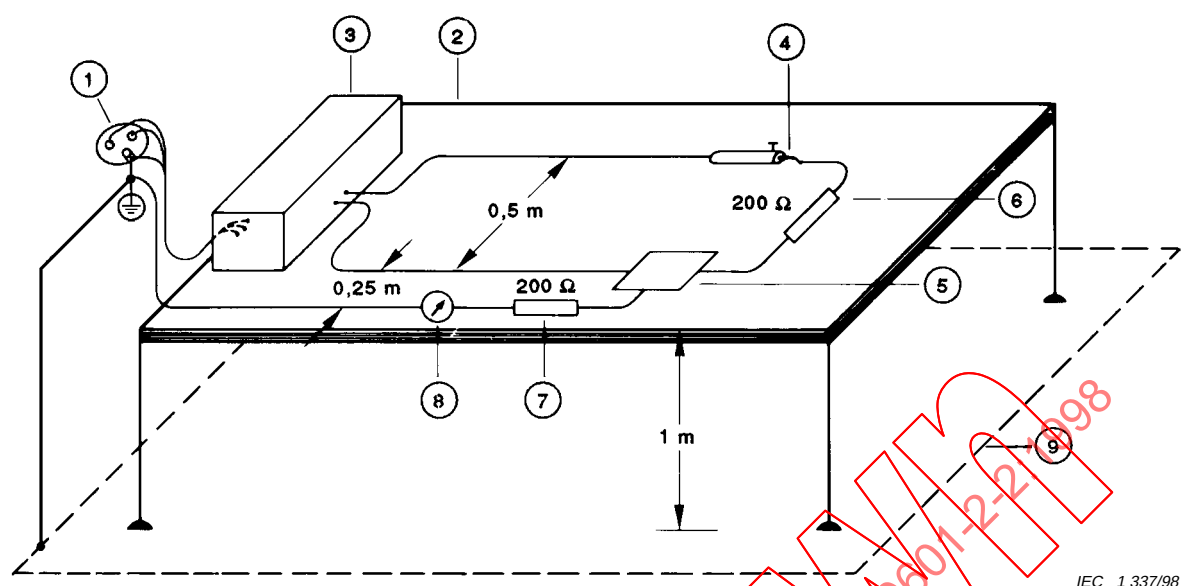
Figure 101 – Measurement of h.f. LEAKAGE CURRENT with NEUTRAL ELECTRODE referenced to earth, and load between electrodes (see test 1 of 19.3.101 a) 1))
