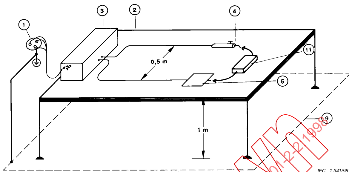
Figure 105 – Measurement of OUTPUT POWER – Monopolar output (see 50)
