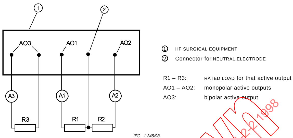
Figure 109 – Method of testing feedback from one active output to another in simultaneous activation (see 46.103 and 51.102)
