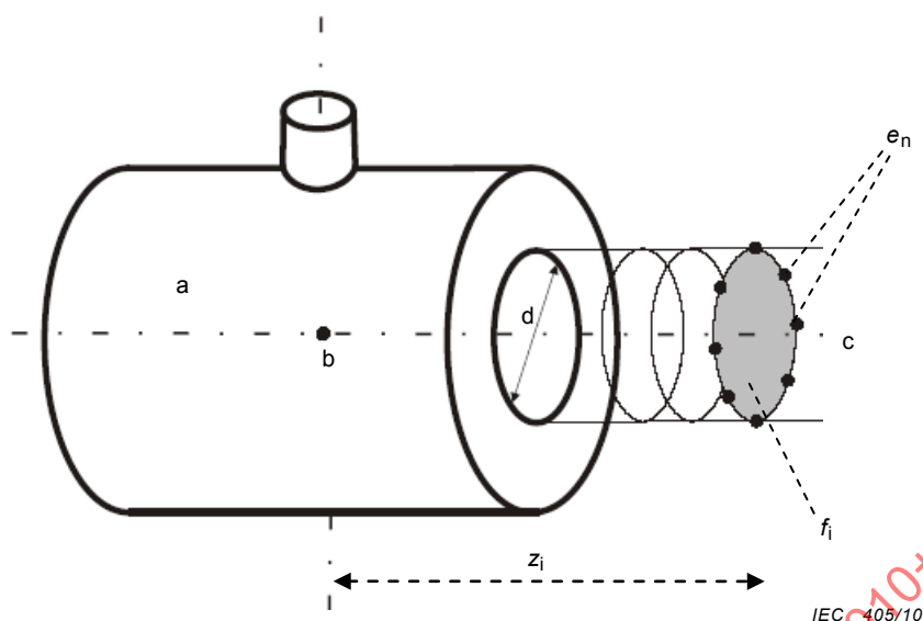
Figure 201.104a – Aimant cylindrique
