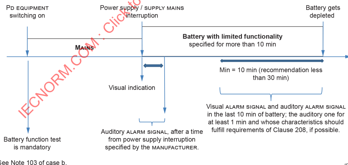
Figure AA.3 – Alarm before battery for limited functionality gets depleted (10 min minimum)
