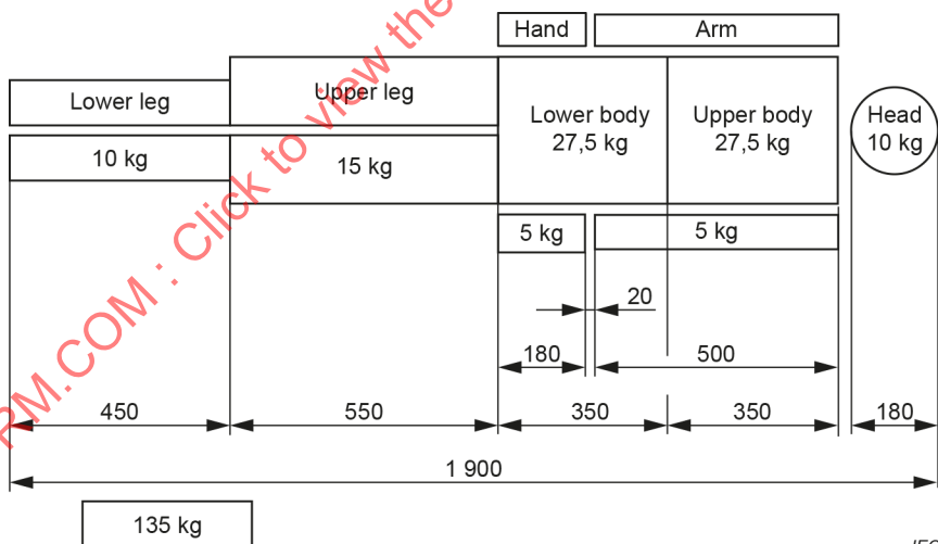
Figure AA.1 – Recommended distribution of mass in excess of 135 kg and examples of application
