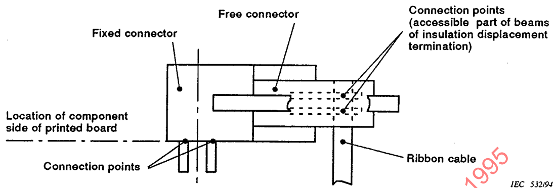
Figure 14 – Connection points for measuring contact resistance
