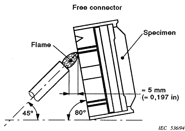
Figure 18 – Free connector arrangement
