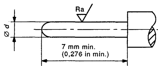
Gauge P2
