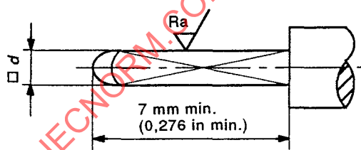
Gauge P1
