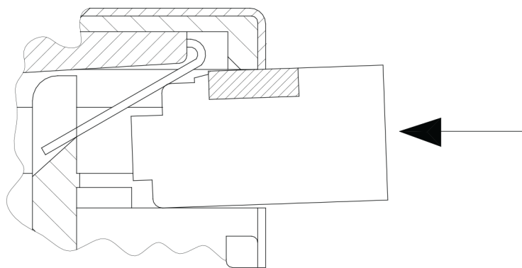
Figure A.2 – Continuity gauge insertion
