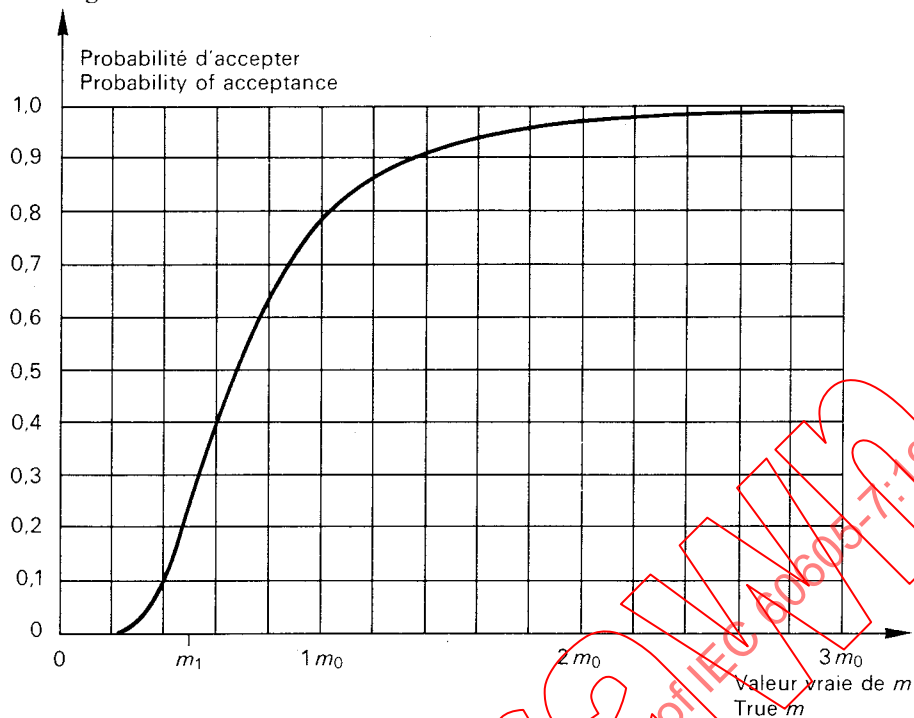
Courbe d'efficacité. Operating characteristic curve.
