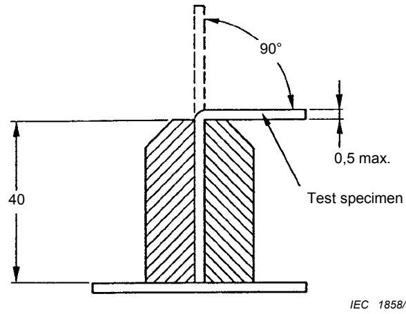
Figure 2 – Bending of test pieces
