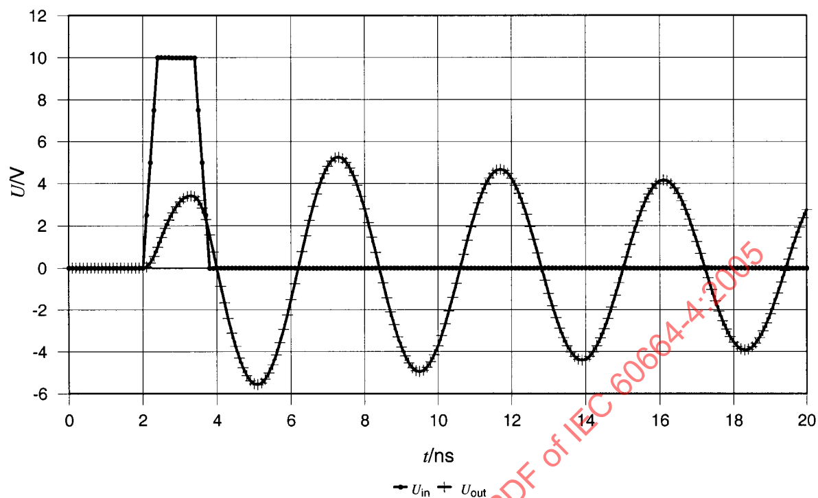
Figure D.7a – PD impulse voltage source
