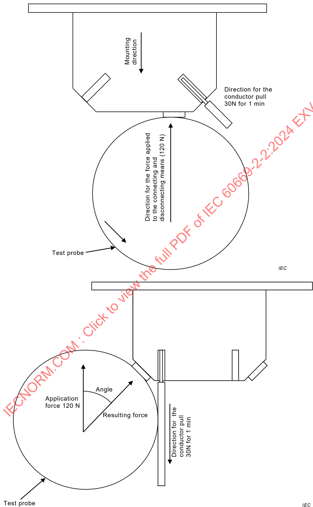
Figure 22b – Test set up
