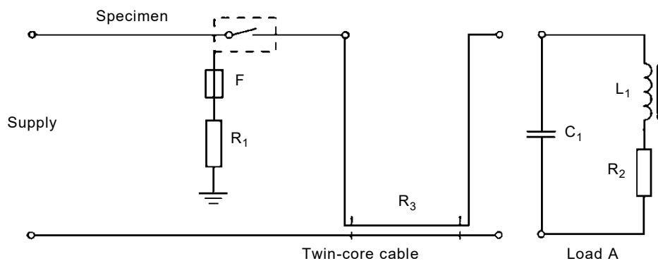
Figure 12a – Circuit diagrams for testing switches for use on externally ballasted lamp loads
