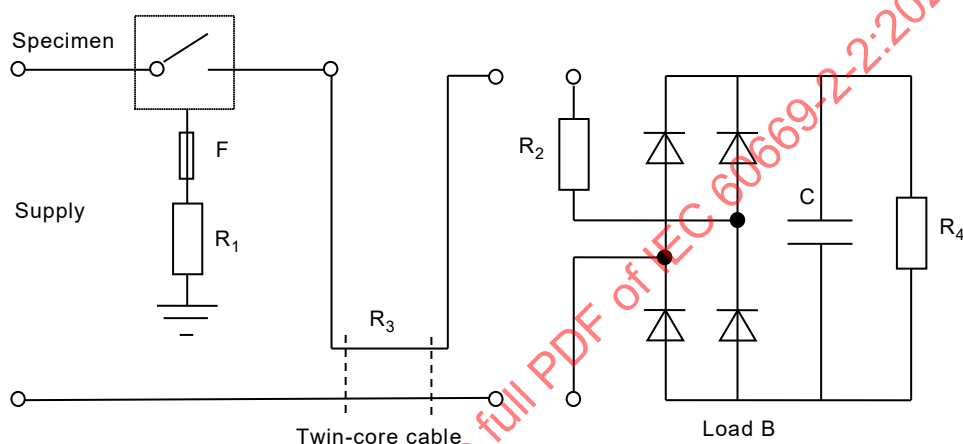
Figure 12a – Circuit diagrams for testing switches for use on externally ballasted lamp loads
