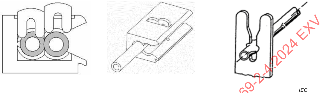
Figure D.1 – Example of insulation-piercing terminals
