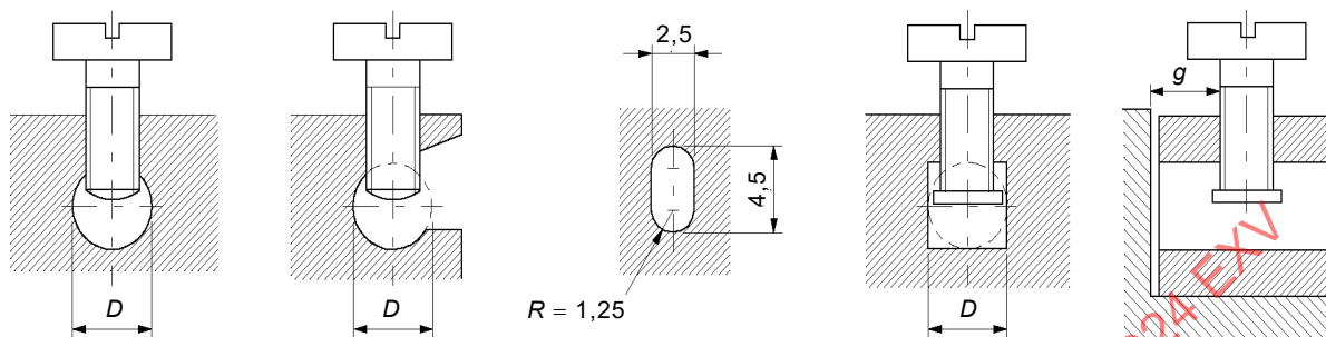
Elongated hole terminal
