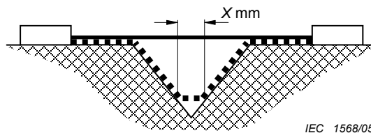
Figure AA.2 – Wide groove
