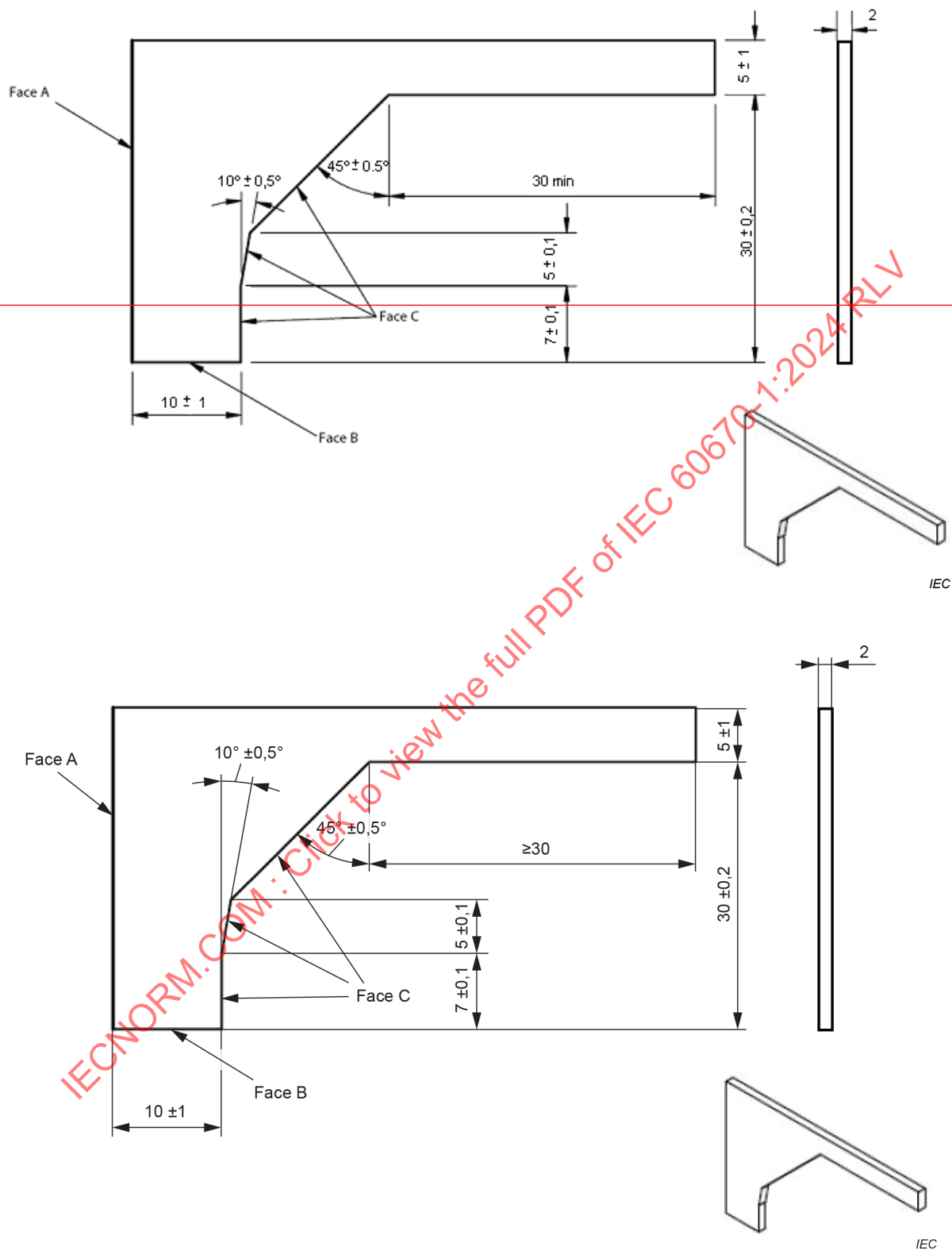
Figure 7 – Gauge for the verification of the outline of lids, covers or cover-plates
