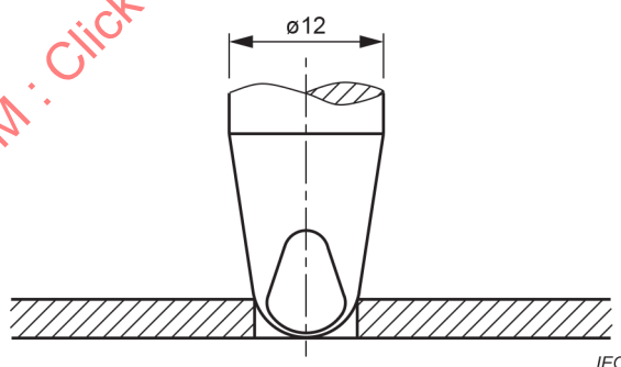
Figure 3 – Demonstration of the non-penetration of the internal volume
