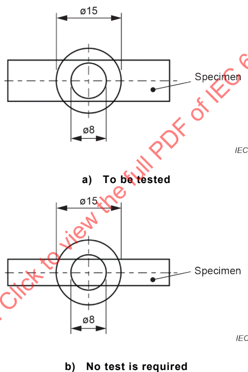
Figure 27 – Diagrammatic representation of the glow-wire test
