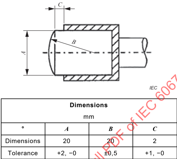
Figure 2 – Test piston dimensions
