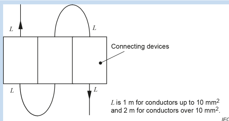
Figure 102 – Multiway terminal device
