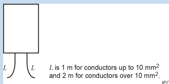
Figure 101 – Single terminal device
