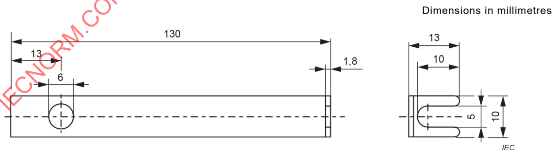
Figure 5 – Test strap
