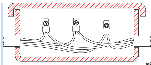
Figure AA.1 – Four examples of connecting boxes/enclosures
