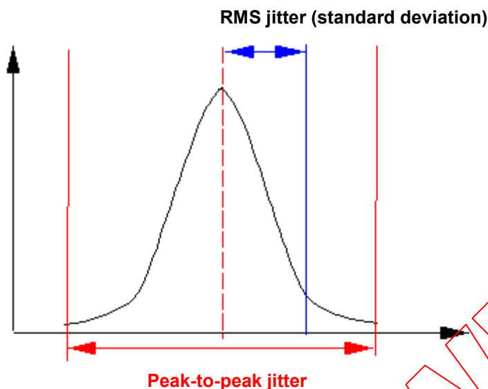
Figure 2 – Explanatory diagram of the amount of jitter applied to r.m.s. jitter
