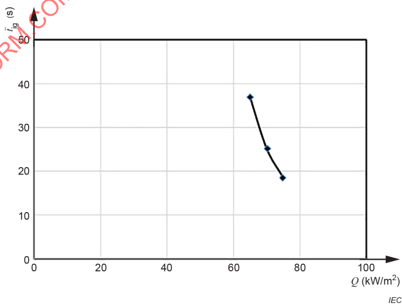
Figure B.3 – Ignition times for HIPS (example)
