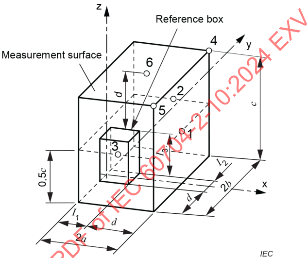
Figure 2 – Measurement surface – parallelepiped – with key microphone positions, for floor standing appliances placed against a wall
