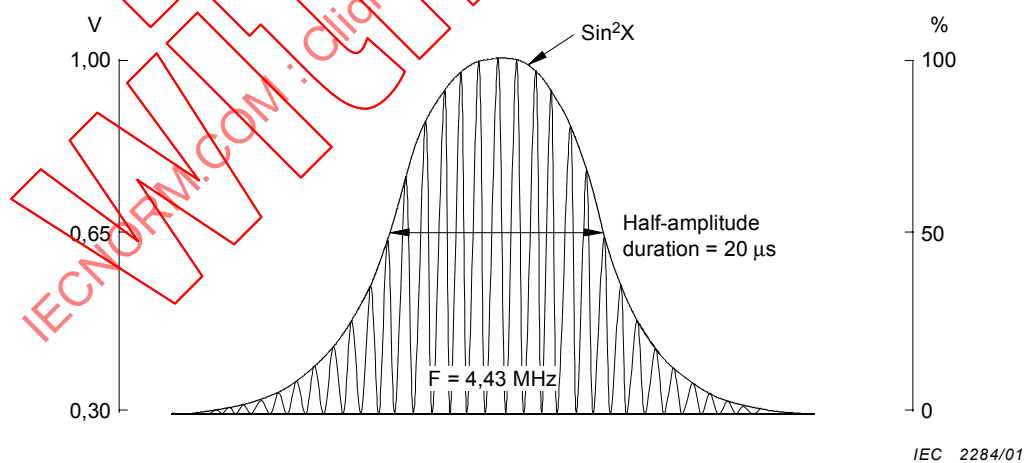
Figure 7 – Test signal (signal F for 625 line systems) employed for chrominance/luminance gain and delay inequality
