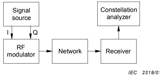
Figure 34 – Test set-up for modulation error ratio (MER) measurement and phase jitter measurement
