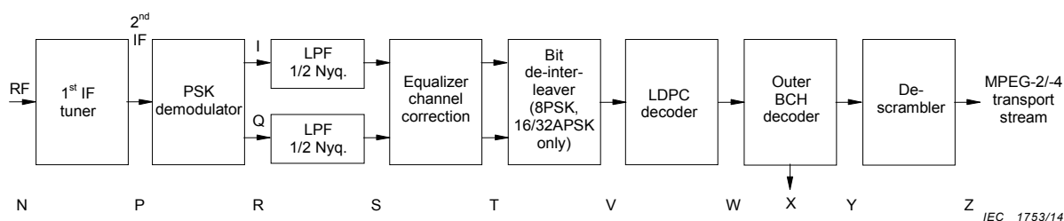
Figure 32 – Reference receiver for DVB-S2 demodulation (QPSK, 8PSK, 16APSK, 32APSK)
