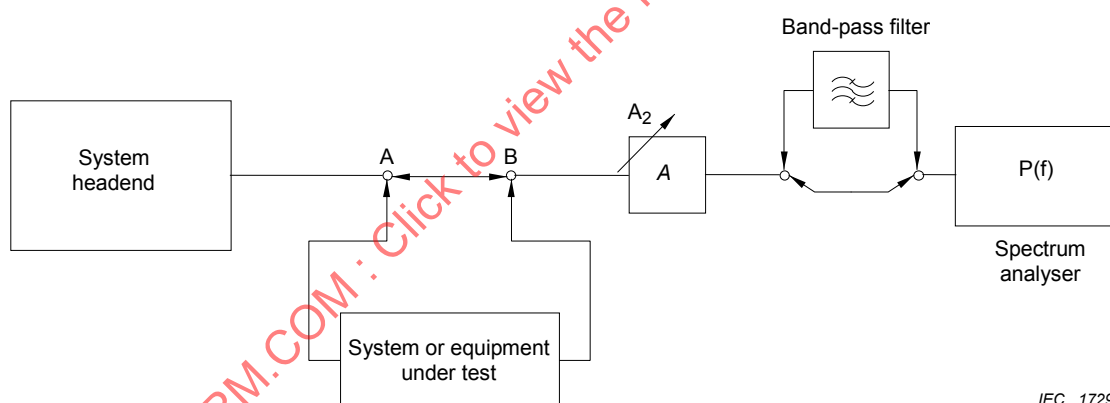
Figure 9 – Connection of test equipment for the measurement of non-linear distortion by composite beat
