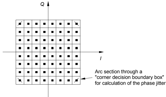
Figure 42 – Example of constellation diagram for a 64 QAM modulation format with arc sections due to phase jitter
