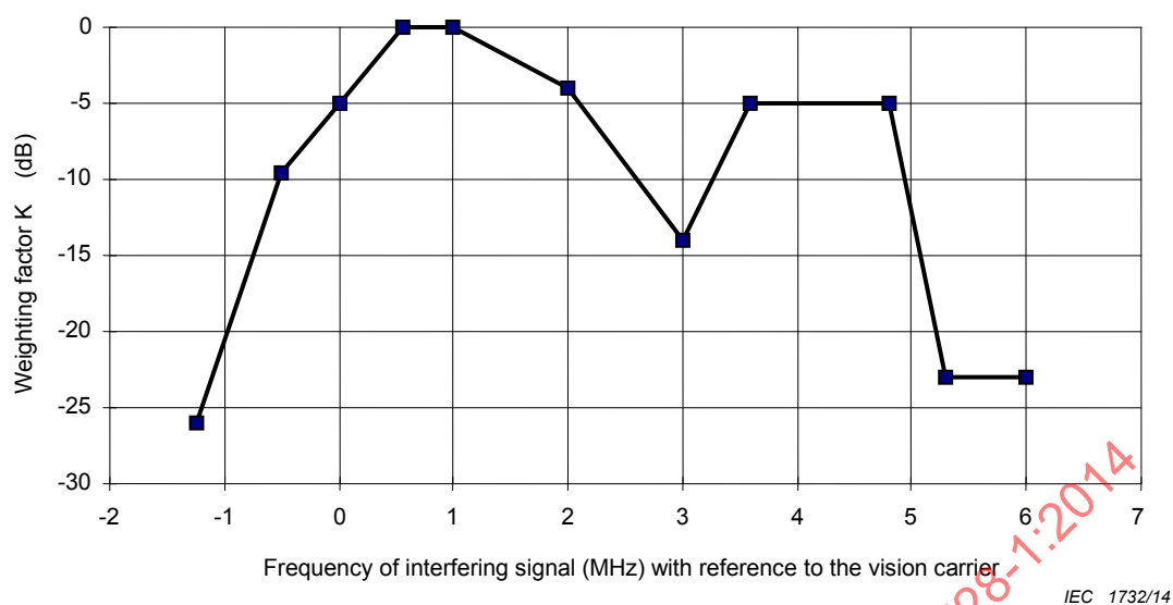
Figure 12 – Weighting curve for 625-line systems D and K (PAL): CW interference with no special (frequency offset) control
