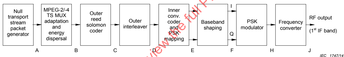
Figure 26 – PSK modulation (QPSK, BPSK or TC8PSK)
