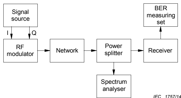
Figure 36 – Test set-up for BER measurement
