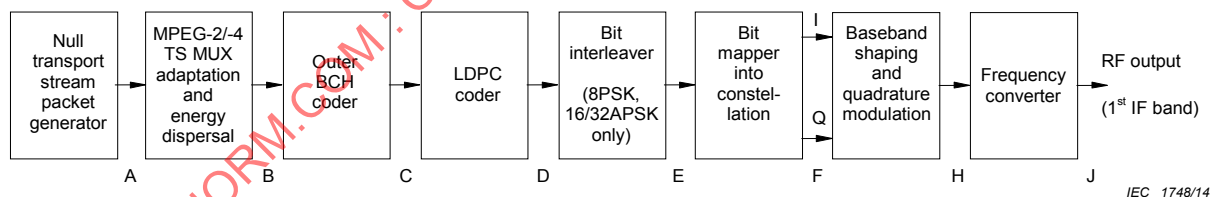
Figure 27 – DVB-S2 modulation (QPSK, 8PSK, 16APSK, 32APSK)
