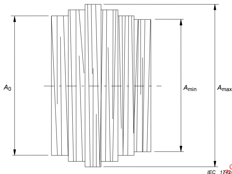
Figure 21 – Example of the modified staircase waveform
