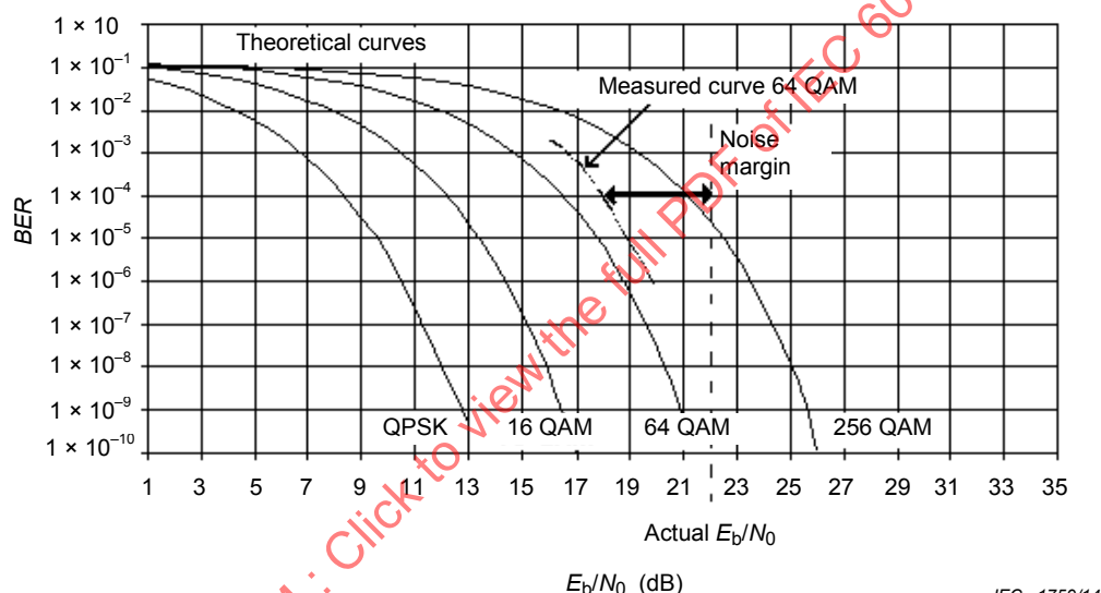
Figure 38 – Example of BER measurement versus E_b/N_0
