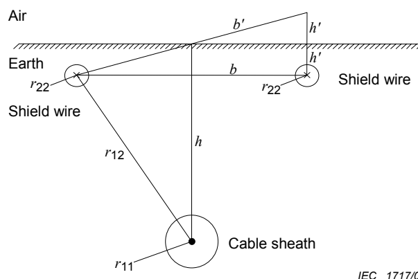
Figure B.2 – Principle of two shield wires
