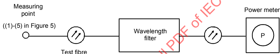
Figure 7 – Measurement of optical power using a wavelength filter
