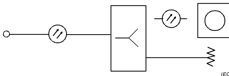
Figure 6 – Measurement of optical power using a WDM coupler
