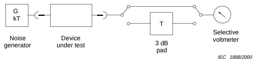
Figure 8 – Measurement of noise figure
