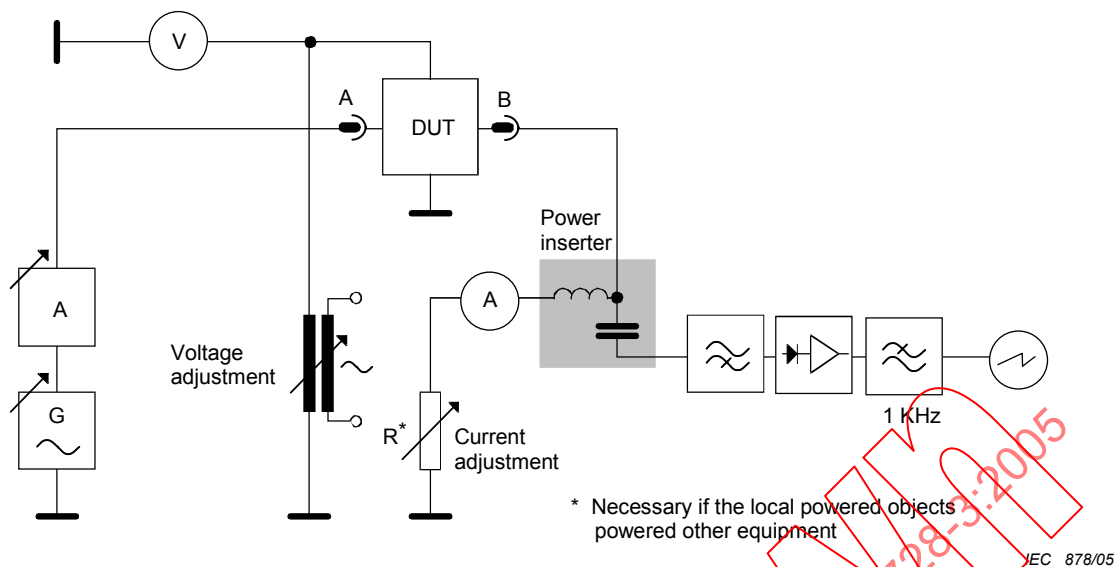
Figure 7 – Test set-up for local-powered objects
