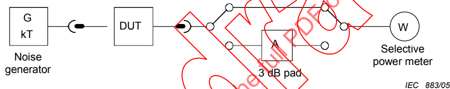
Figure 12 – Measurement of noise figure
