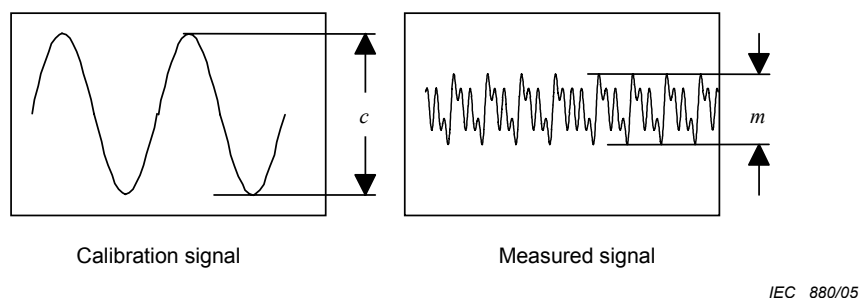
Figure 9 – Oscilloscope display
