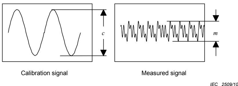
Figure 9 – Oscilloscope display
