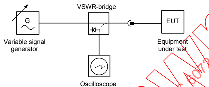
Figure 2 – Measurement of return loss
