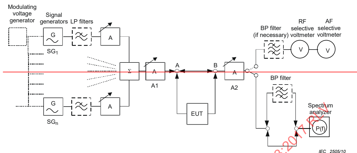
Figure 5 — Connection of test equipment for the measurement of composite crossmodulation
