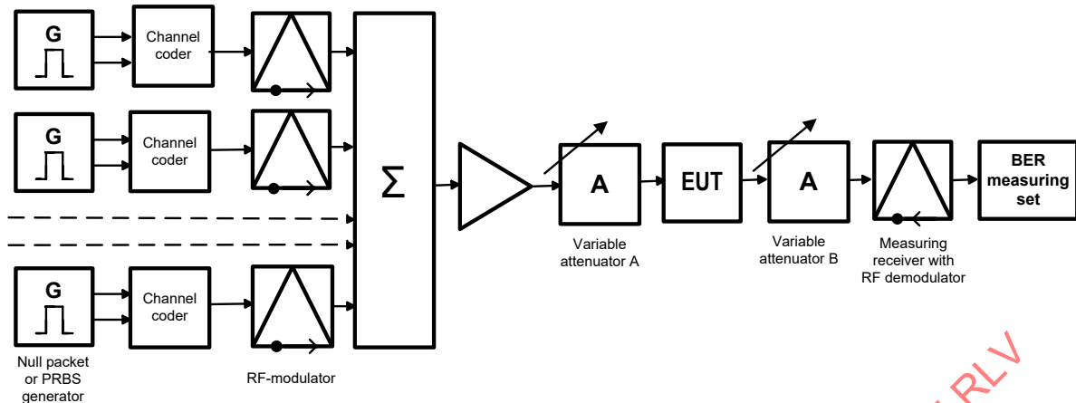
Figure 3 – BER measurement test configuration
