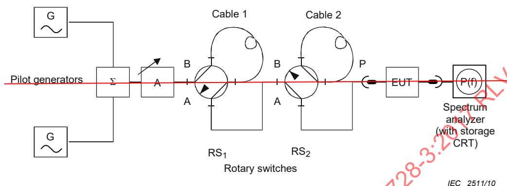
Figure 11 — Measurement of AGC step response
