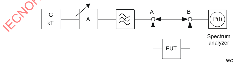
Figure 13 – Test setup for the non-linearity measurement
