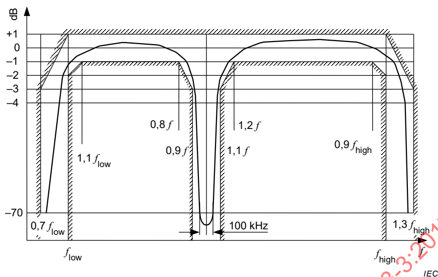
Figure 12 – Characteristic of the noise filter
