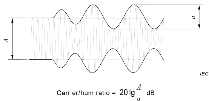
Figure 6 – Carrier/hum ratio
