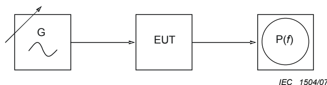
Figure 17 – Test set-up for phase noise measurement
