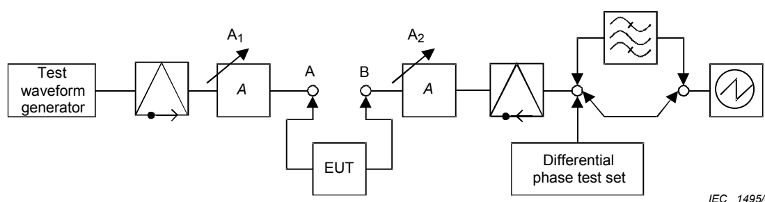
Figure 9 – Arrangement of test equipment for measurement of differential gain and phase
