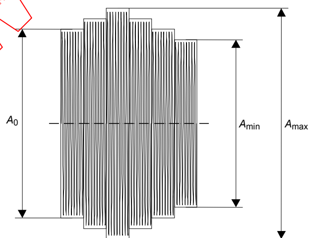
Figure 11 – Example of modified staircase
