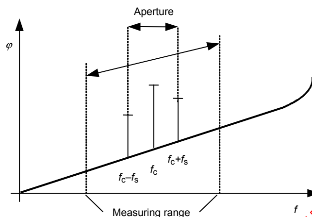
Figure 14 – Spectral presentation of the group delay measurement
