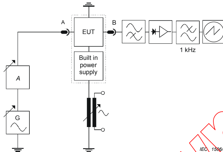
Figure 20 – Test set-up for equipment with built-in power supply
