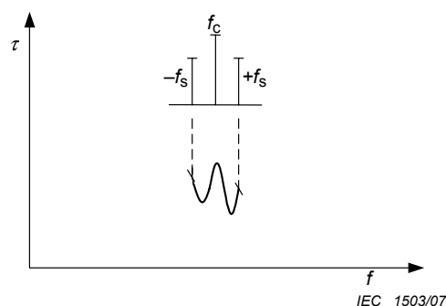
Figure 16b – Surface acoustic wave filter: Group delay ripple measured with too high split frequency
