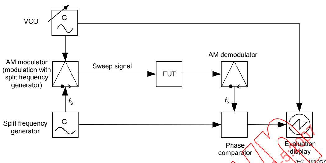
Figure 15 – Description of the measuring set-up
