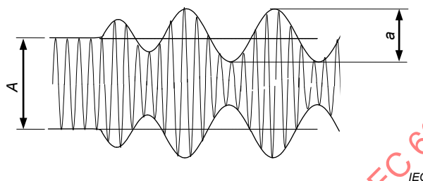
Figure 21 – Carrier/hum ratio
