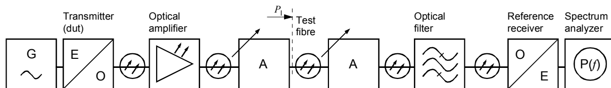
Figure 22 – Arrangement for measuring the SBS threshold
