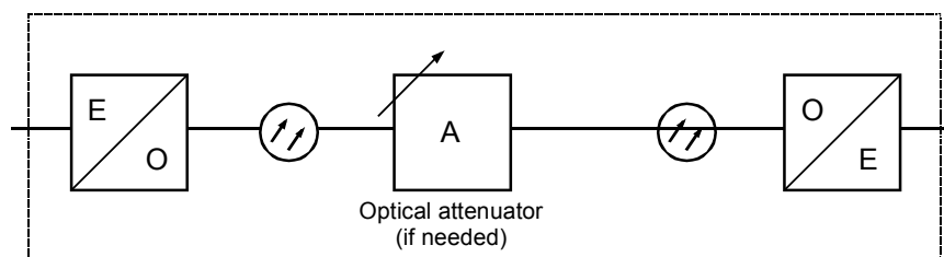
Figure 13 – Device under test for measuring CSO of optical transmitters
