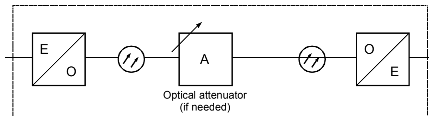
Figure 14 – Device under test for measuring CTB of optical transmitters
