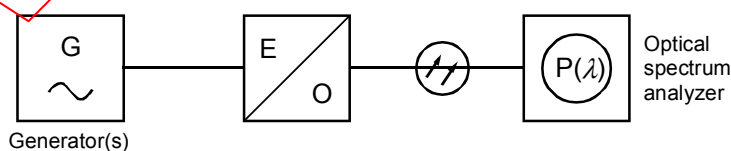
Figure 6 – Measurement of central wavelength and spectral width under modulation
