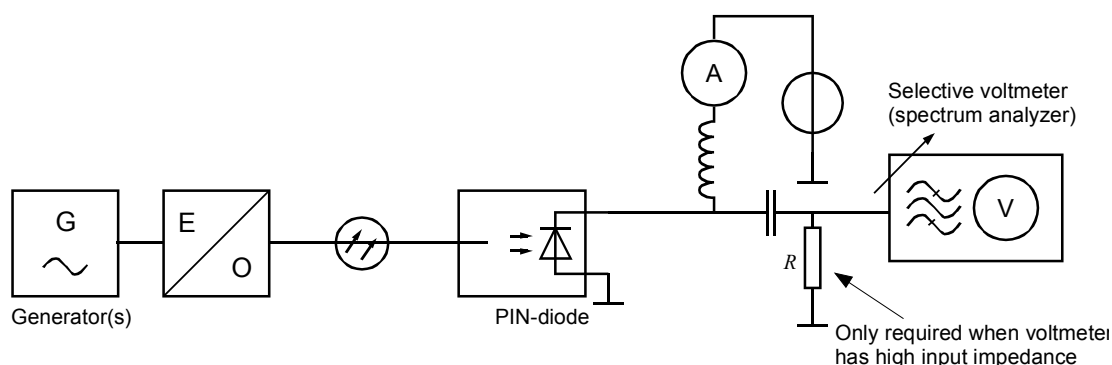
Figure 8 – Measurement of the optical modulation index
