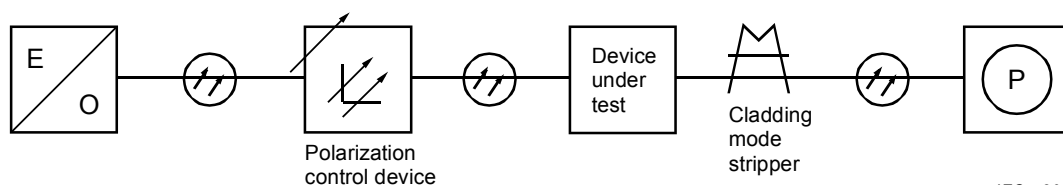
Figure 5 – Measurement of the polarization dependent loss
