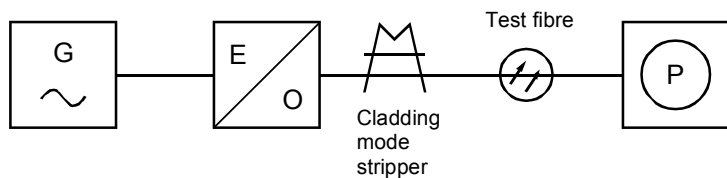
Figure 1 – Measurement of optical power
