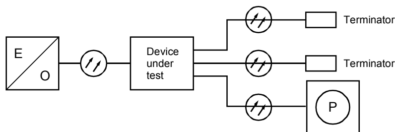
Figure 2 – Measurement of optical loss, directivity and isolation
