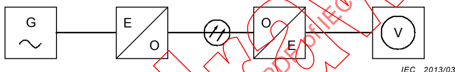
Figure 10 – Measurement of the frequency range and flatness
