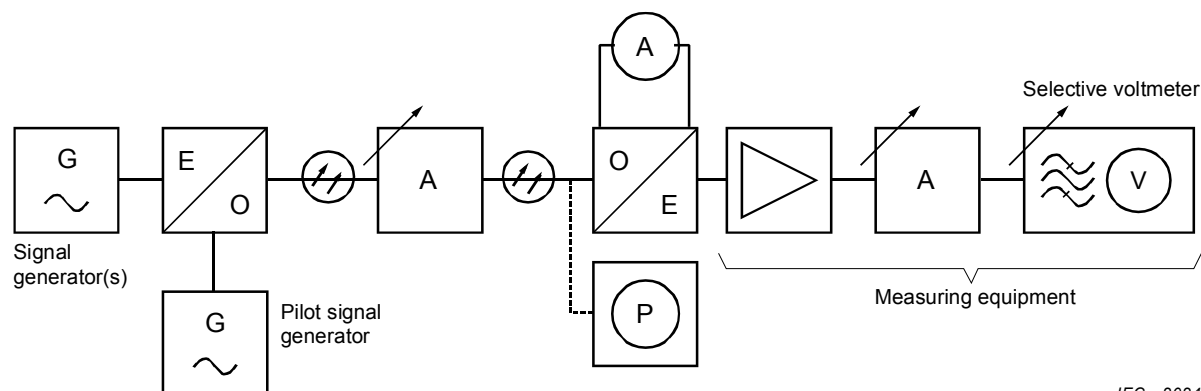
Figure 21 – Measurement set-up for determination of the noise parameters and the optical modulation index
