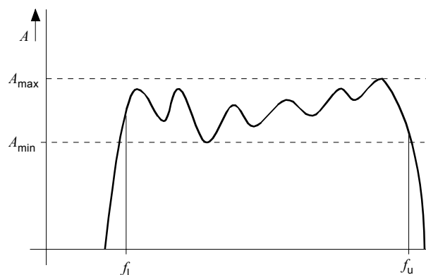
Figure 12 – Evaluating the flatness
