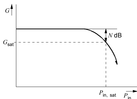
Figure 4 – Optical saturation output power
