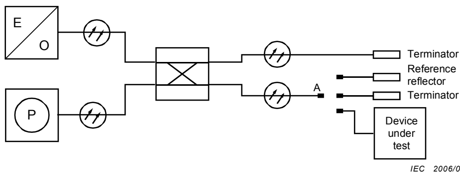
Figure 3 – Measurement of the optical return loss
